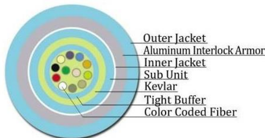
Aluminum Interlocking Armor (AIA)
