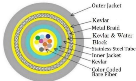
24F 250um Fiber, Kevlar, Jacket, Steel Tube, Kevlar & Water Block, Metal braid, Kevlar, Outer Jacket, UL/OFCP
