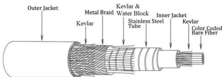
Outer Jacket Material: Plenum Color: Black Outer Diameter: 6.5 mm
