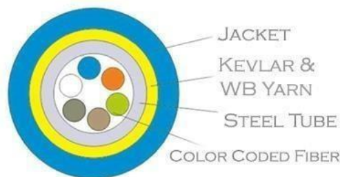
0.9mm Color Coded Fiber, Steel Tube, Kevlar, Water Block Yarn, Outer Jacket (Black), UL/OFCP
